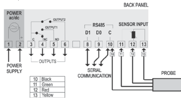
Fig. 2 - N322RHT terminals
